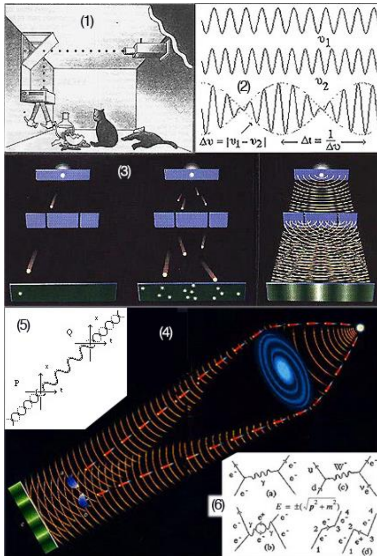
Fig 6: (1) Schrodinger cat experiment has a cat in a box with a radioactive scintillation counter, which works by quantum tunneling out of the nucleus triggering a hammer to smash a cyanide flask pronouncing a cat alive and dead with differing probabilities according to the tunneling wave function of the nucleus potential well. However we find the cat is either alive or dead with certainty. (2) The uncertainty relation \Delta E \Delta t \approx h is derived directly from the counting of wave coherence beats, since energy is related to frequency by E = h\nu and \Delta t \approx 1 / \Delta \nu . (3) Quantum interference experiment shows wave-particle complementarity and reduction of the wave packet occurs statistically (centre) according to the amplitude of the wave function (right) although the wave-particle reduction of individual quanta (left) is unpredictable. (4) Wheeler delayed choice shows time reversed boundary condition. A cosmic scale version of the interference experiment using galactic gravitational lensing can be adjusted at the detector after the photons have traversed space to either sample a particle going one way round, or a wave interference going both ways. (5) The transactional interpretation visualizes an exchanged particle wave function as the interference of a retarded usual time direction offer wave and a time-reversed advanced confirmation wave. (6) Time symmetric interactions also occur in quantum field theories where special relativity allows both advanced
