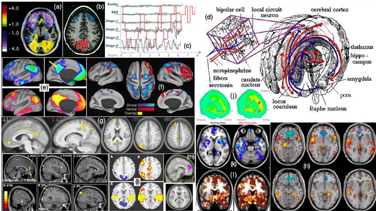
Fig 2: Physiological underpinnings of a variety of brain states. (a,b) fMRI and PET scans of REM (dreaming) sleep show increased occipital (visual) activity and reduced prefrontal (executive) function, with an EEG similar to the waking brain (Braun). (c) Sleep phases of REM and non-REM sleep alternate in waves. The EEGs are on a time scale of seconds, the sleep waves in hours. (d) Sleep phases are driven by ascending serotonin and nor epinephrine pathways from the Raphe nucleus and Locus coeruleus. (e) The default network associated with worry and recollection of events to prepare for the future shows depression of activity during task performance and increase during rest (Raichle et al, Raichle & Snyder, Mason et al, Fox D, Horowitz et al, Buckner et al, Marshall). (f) There are believed to be two attention systems in the human brain (Fox et al.) a bilateral dorsal attention system (blue) involved in top-down orienting of attention and a right-lateralized ventral attention system (red) involved in reorienting attention in response to salient sensory stimuli. (g) Zen meditation studies (Pagnoni et al, Ritskes et al) in which subjects are asked to switch from a verbal task to contemplation show transient activity consistent with the default network which is more quickly suppressed by experienced meditators more effectively inhibiting verbal thought. (h) Carmelite nuns entering oneness with God show fMRI activations in areas in specific frontal, parietal, temporal and basal areas consistent with directed control (Beauregard & Paquette). (i) Tibetan Buddhists performing compassion meditation for other people's suffering show specific activation in limbic regions including cingulate cortex and insula, consistent with an empathic response to another's pain (Lutz et al 2008). (j) PET study of psilocybin taken orally shows frontal activation by comparison with a resting state (Vollenweider et al). (k) fMRI study during the 12 minutes after intravenous administration of psilocybin shows reduced activity in medial frontal cortex (mPFC), posterior cingulate cortex (PCC) and other areas (Carhart-Harris et al 2012a, Lee & Roth) suggesting suppression of the default network as the effects come on. (l) Increases in activity associated with autobiographical memories on psilocybin right over placebo (left) (Carhart-Harris et al. 2012b). (m) Increases in fMRI in frontal and paralimbic brain regions in an ayahuasca session (Riba et al 2006). (n) Above ketamine induces a decrease in ventromedial frontal cortex (blue) and increased activity in mid-posterior cingulate, thalamus and temporal cortical regions (yellow-red) consistent with its dissociative effects. Below inhibition of ketamine activity by lamotrigine, a sodium channel blocker that decreases glutamate release (Deakin et al).
