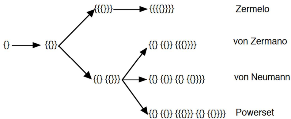
Figure 3. Beginnings of four minimal ω-series
